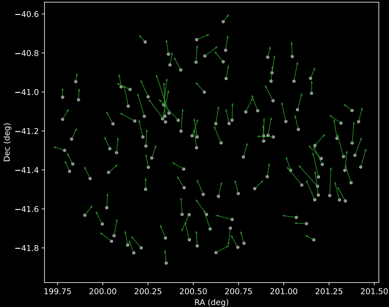
GALAH DR4 Cluster 4 Proper Motion Vectors (n=121)
