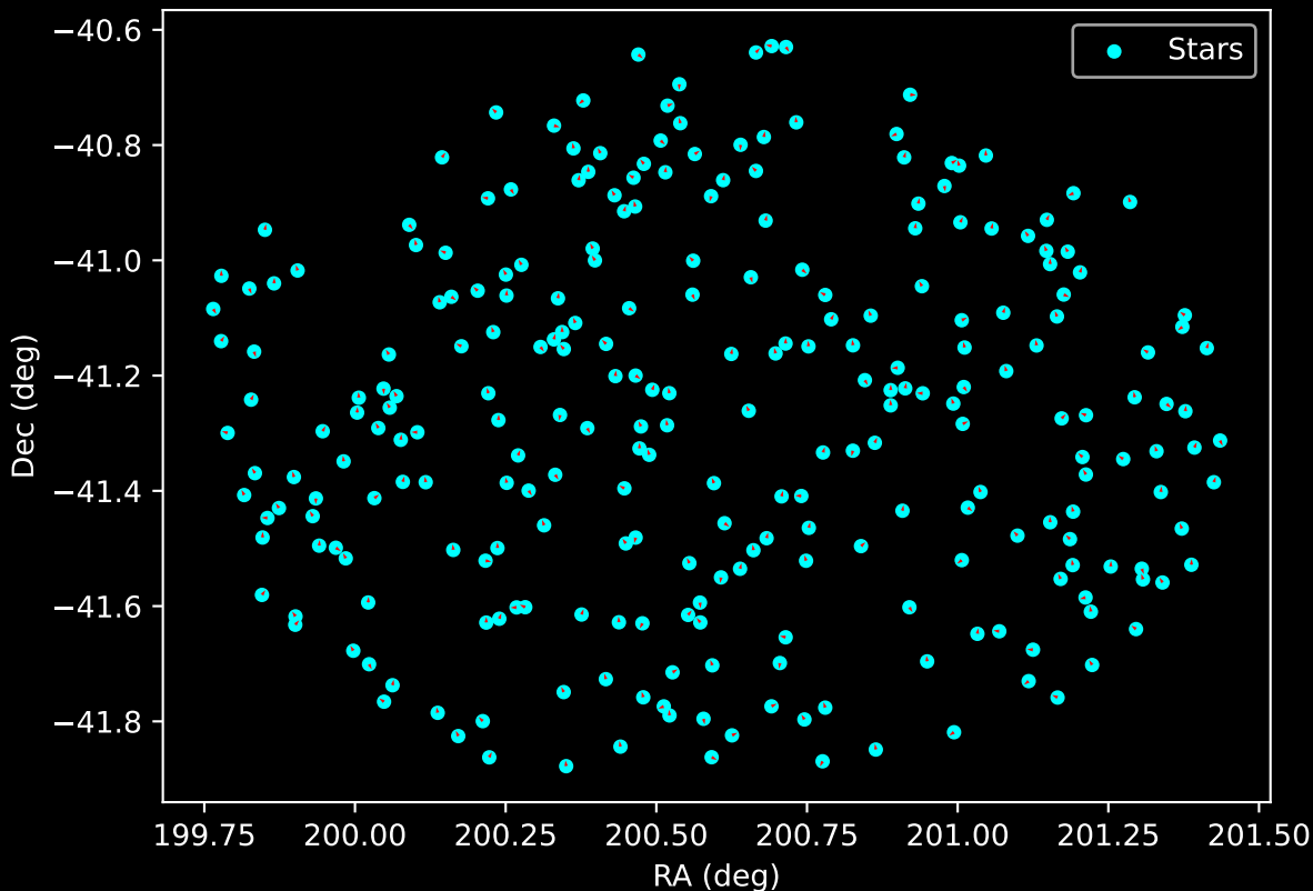
GALAH DR4 Field: [2263] Proper Motion Vectors for Gaia Star Field (n= 261)
