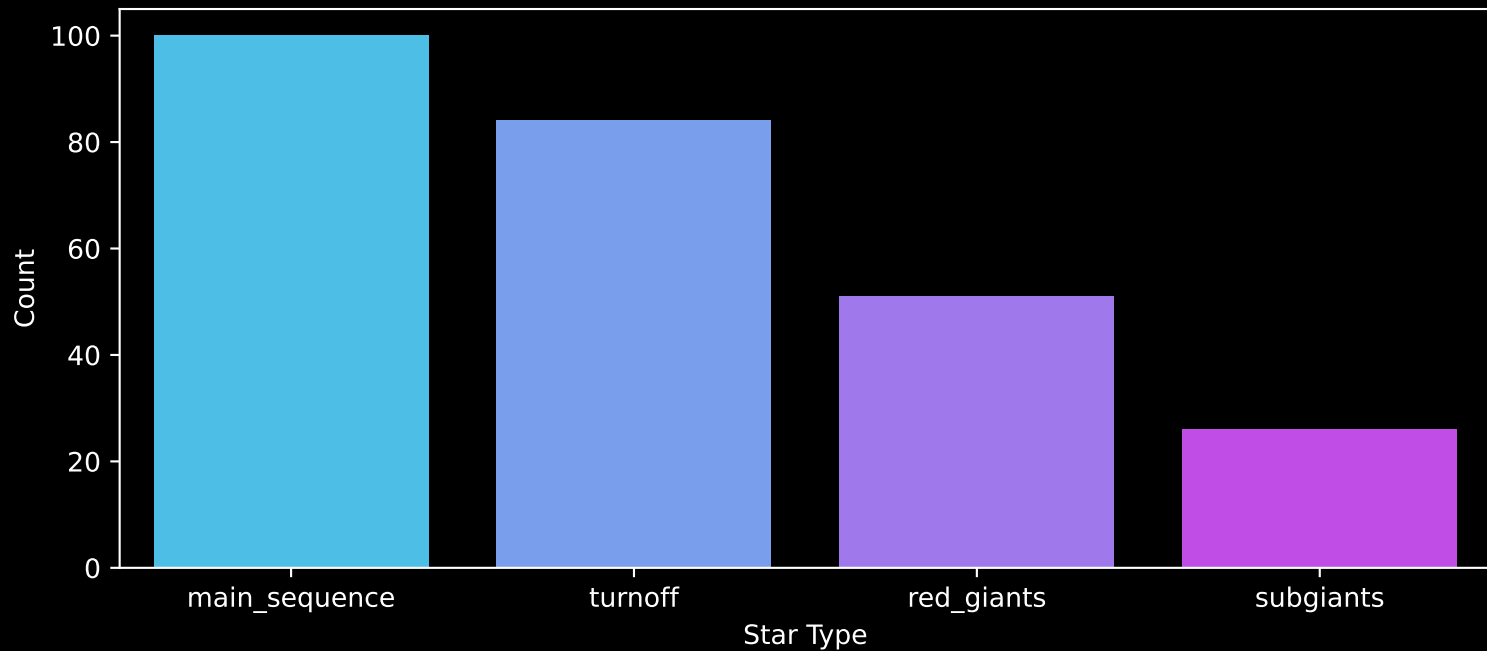
GALAH DR4 Field: [2263] Count plot of Star Type
