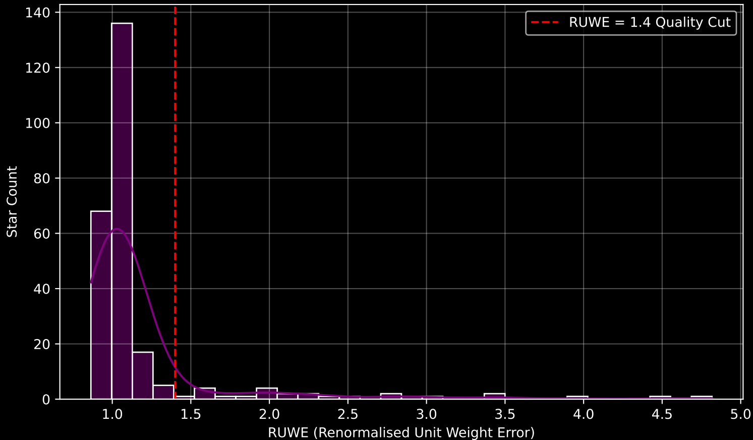
GALAH DR4 Field [2263] RUWE Distribution (n= 252)
